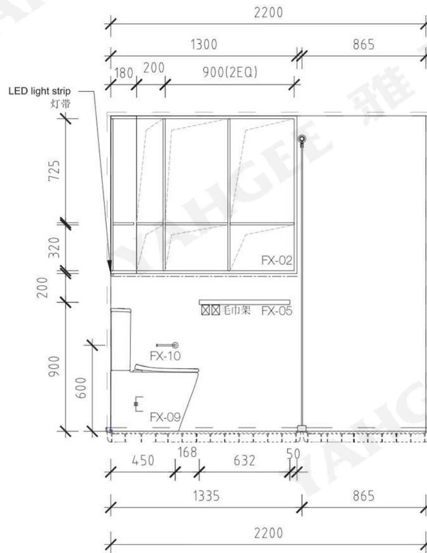
Bathroom Pod Elevation - B
