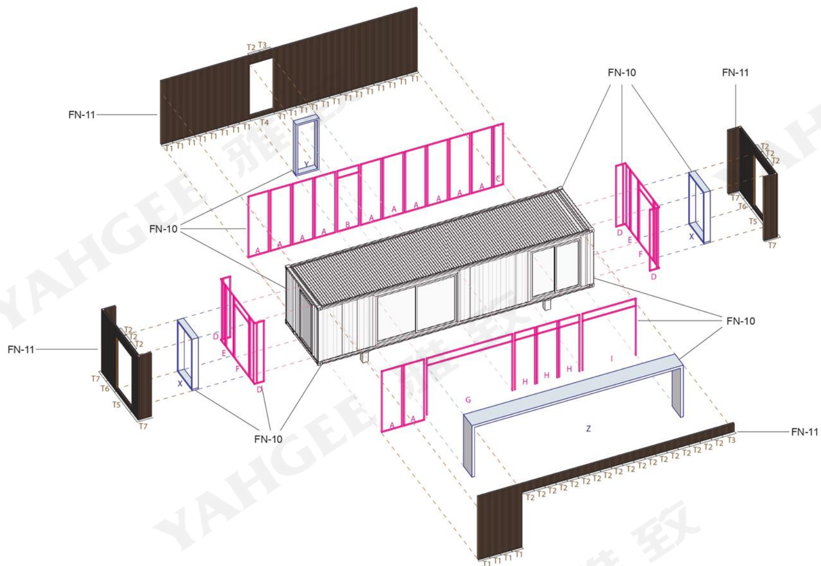
Exploded diagram of overcladding
