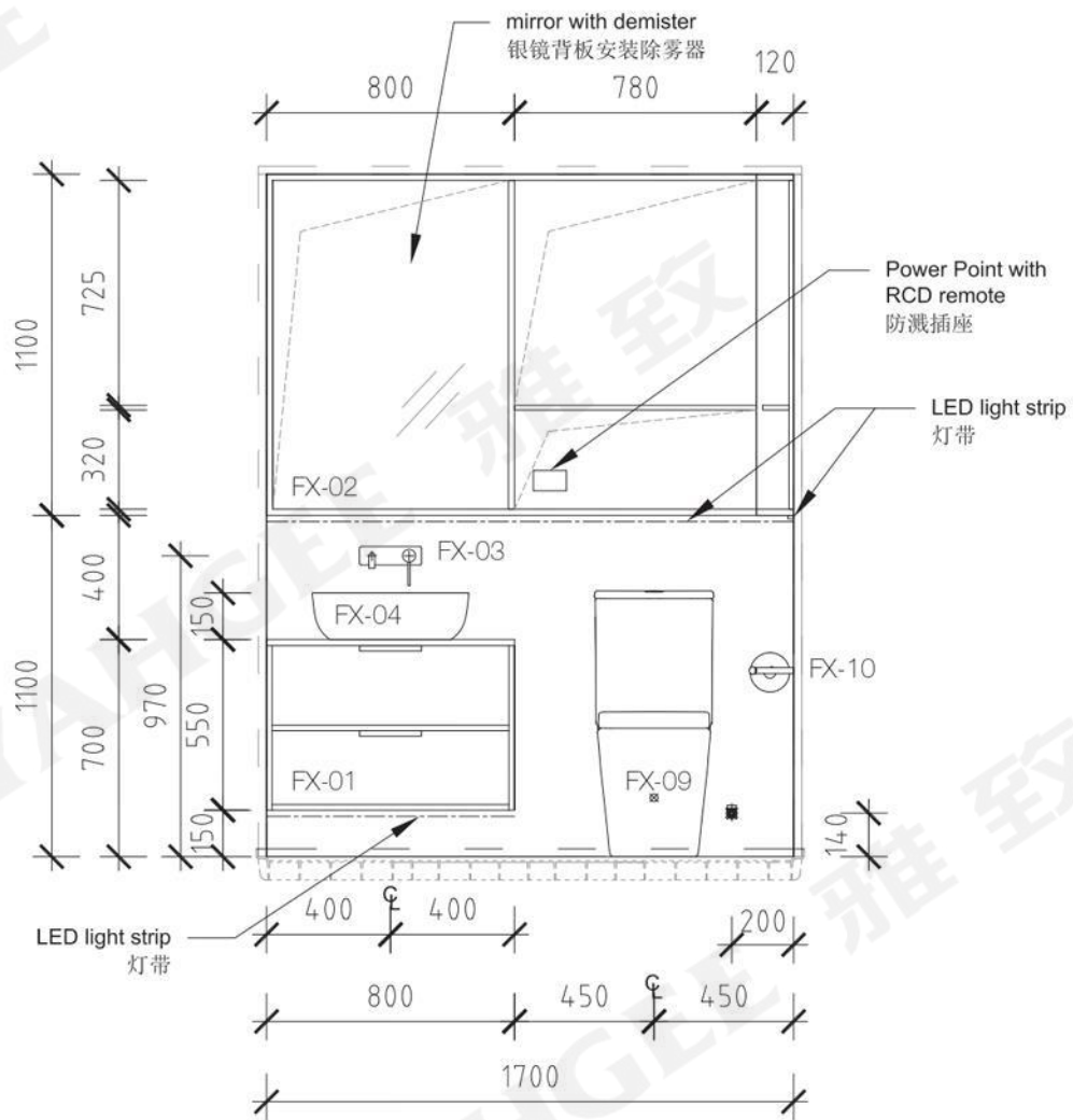
Bathroom Pod Elevation - A
