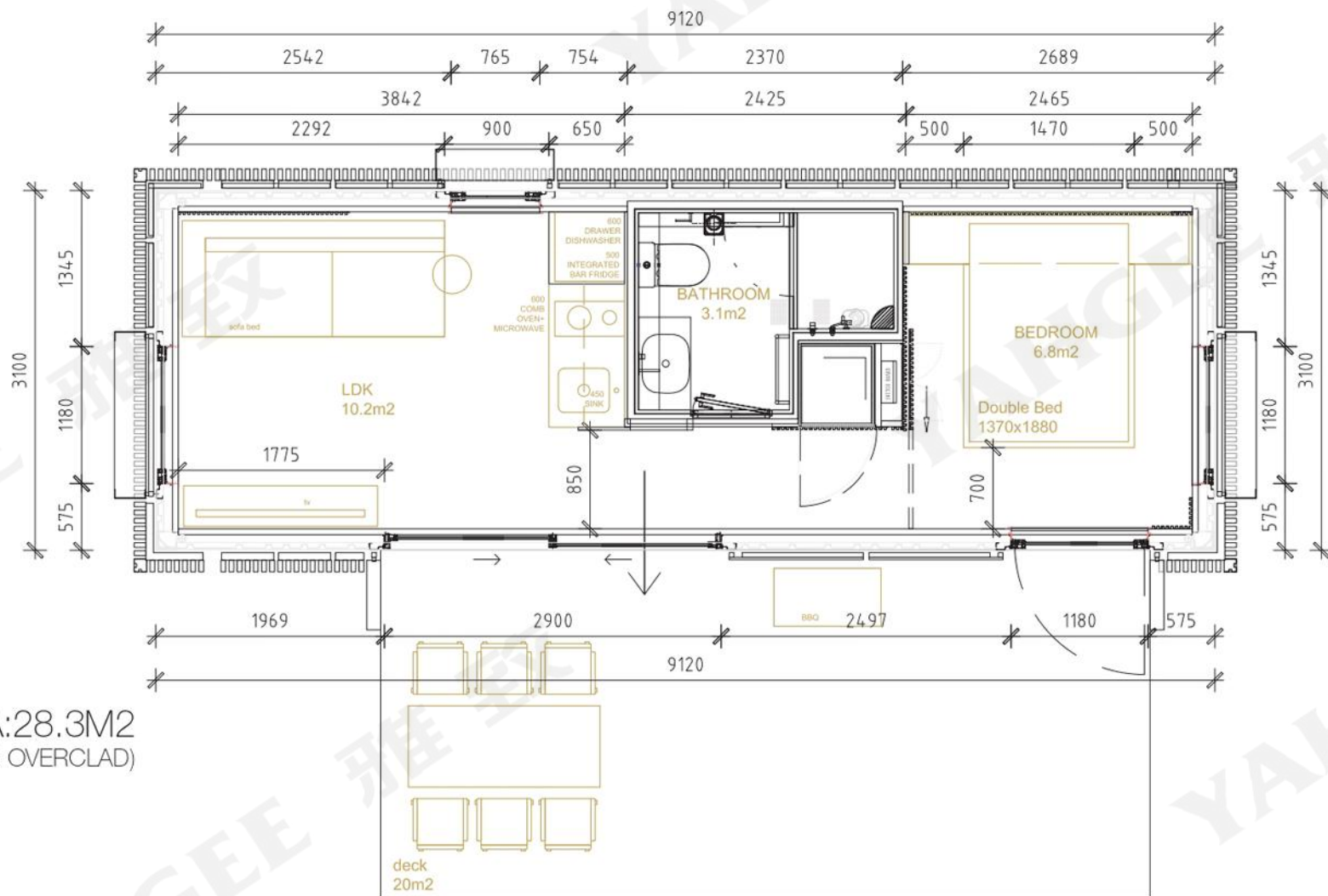
Proposed Layout Plan
